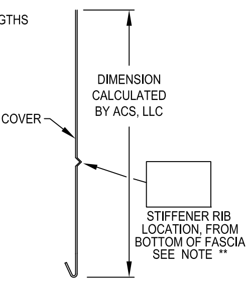
COVER ASSEMBLY
